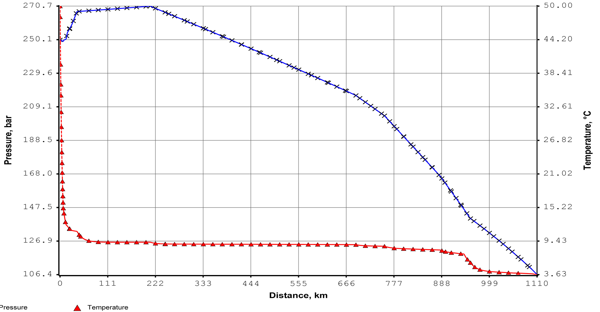
* Pipeline SEALINE1 - Pressure and Temperature Profile -
